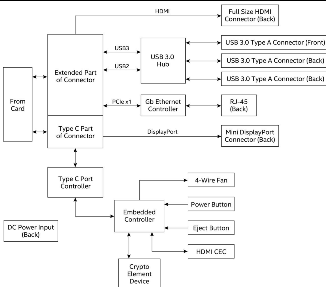
Figure 2. Block Diagram
