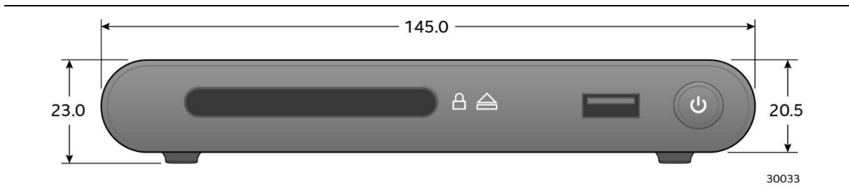
Figure 9. Dock Dimensions – Front View
