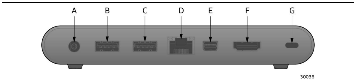
Figure 5. Back Panel Layout
