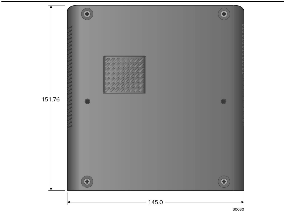
Figure 8. Dock Dimensions – Bottom View
