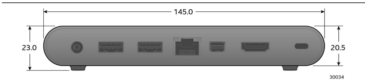
Figure 10. Dock Dimensions – Back View
